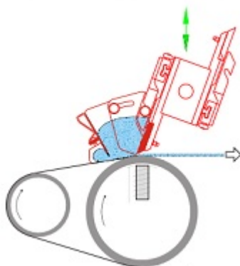
Magnoknife foam application with trough
