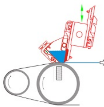
Magnoknife paste application with trough
